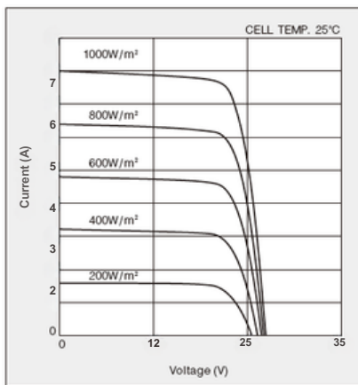
I-V CURVES OF PV MODULE(220W)
